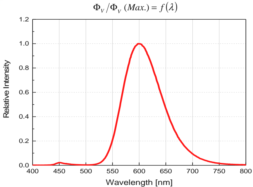
Wavelength Characteristics Relative Spectral Distribution @ T S = 25°C 、 I F = 700mA (PC Amber)
