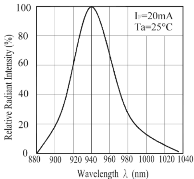
Spectral Sensitivity
