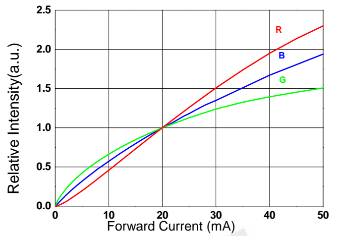
Relative Intensity vs. Forward Current ( T_a=25^{\circ}\text{C} )
