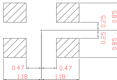
Soldering patterns
