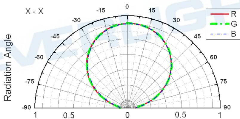
Directivity (Ta=25°C)
