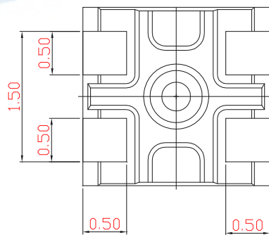
Bot. view
