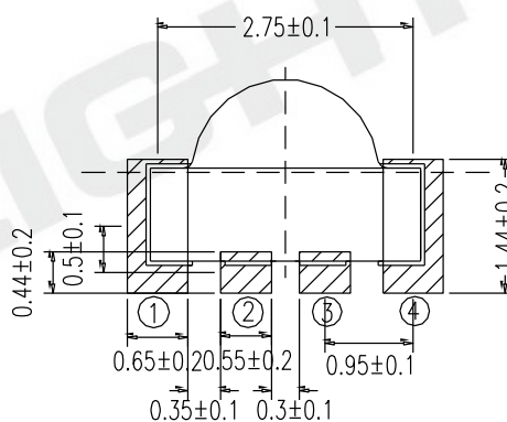
Recommend Soldering Pad
