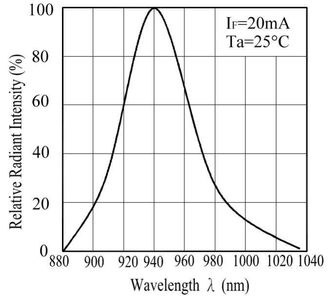
Fig.2 Spectral Distribution
