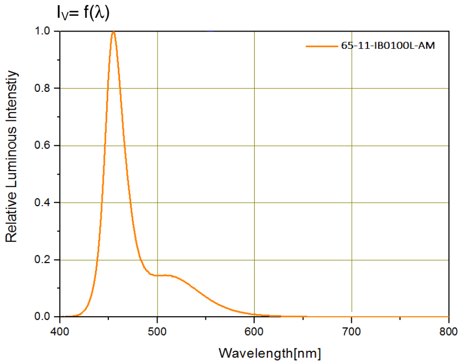
Wavelength Characteristics Relative Spectral Distribution @ Ts = 25°C, If=10mA, RH=30%
