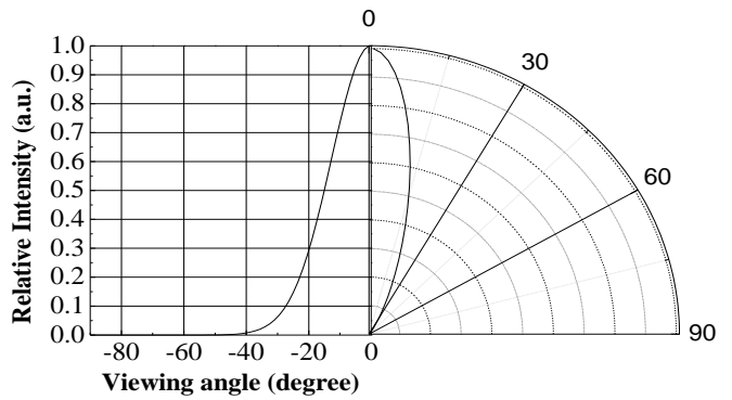
Radiation Characteristics
