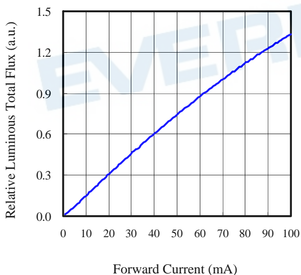
Relative Luminous Total Flux vs. Forward Current (Ta=25°C)
