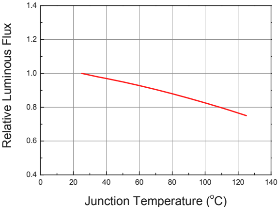
Relative Luminous Flux @ Junction Temperature
