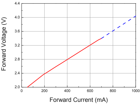
Forward Voltage vs. Forward Current @ T_s = 25^{\circ}\text{C} , 50ms
