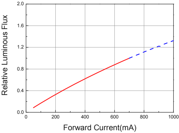
Typical Relative Luminous vs. Forward Current @ T_s = 25^{\circ}\text{C} , 50ms
