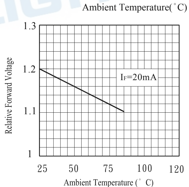
Fig.8 Relative Forward Voltage vs.
