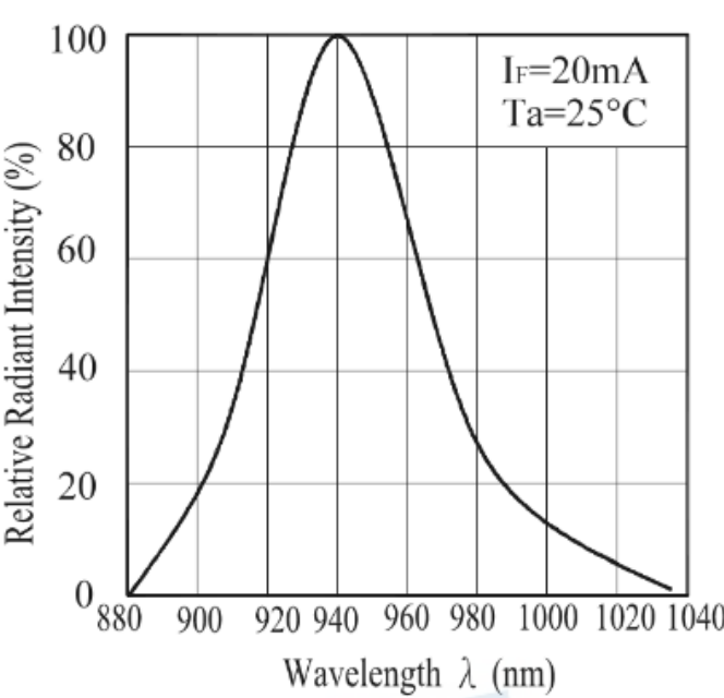
Spectral Sensitivity
