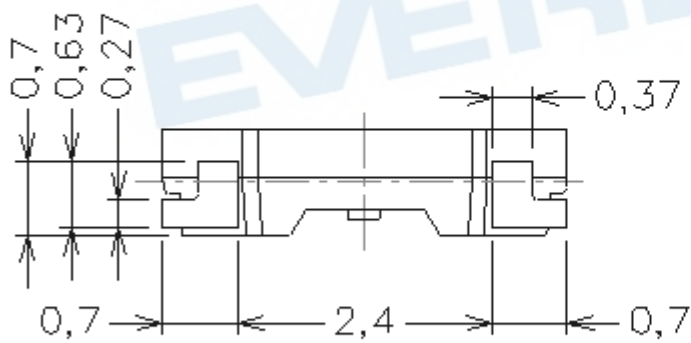
Bot. view
