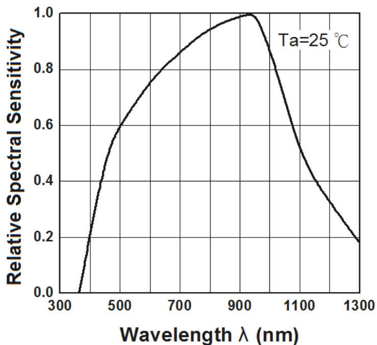
Fig.1 Spectral Sensitivity
