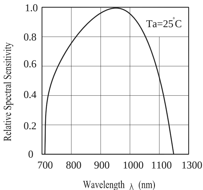
Fig.1 Spectral Sensitivity
