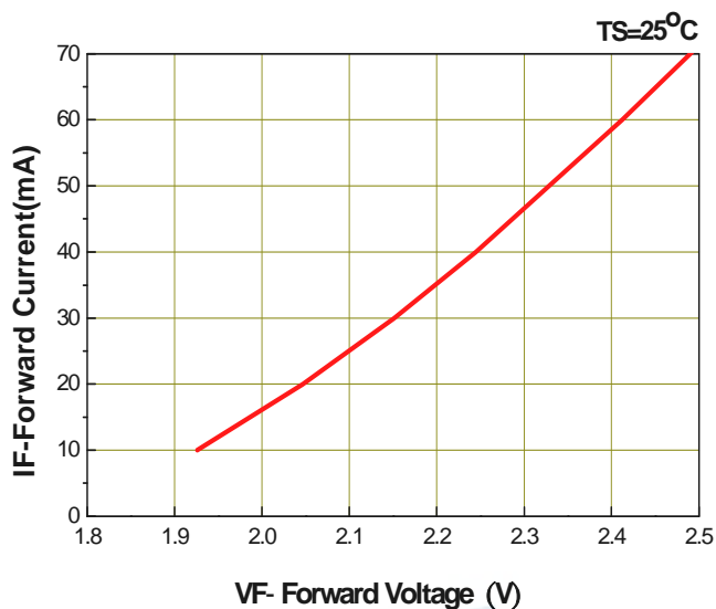
Fig.4 - Forward Current vs. Forward
