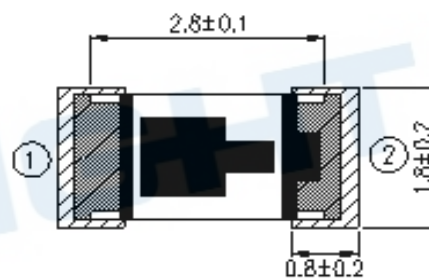
Recommend Soldering Pad
