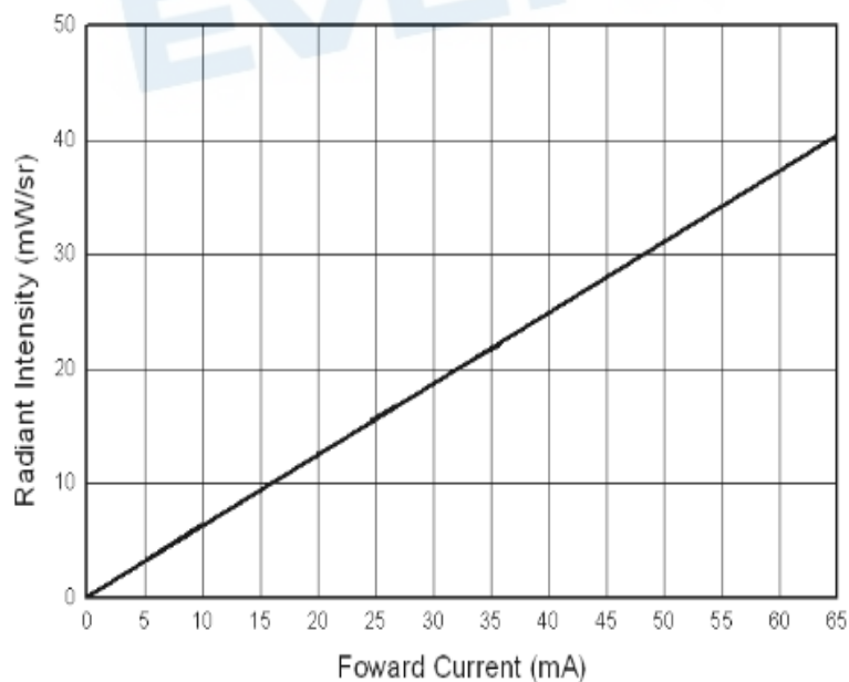
Fig.3 Relative Intensity vs. Forward Current
