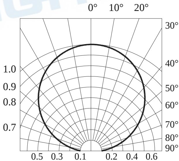
Fig.6 - Radiation Diagram
