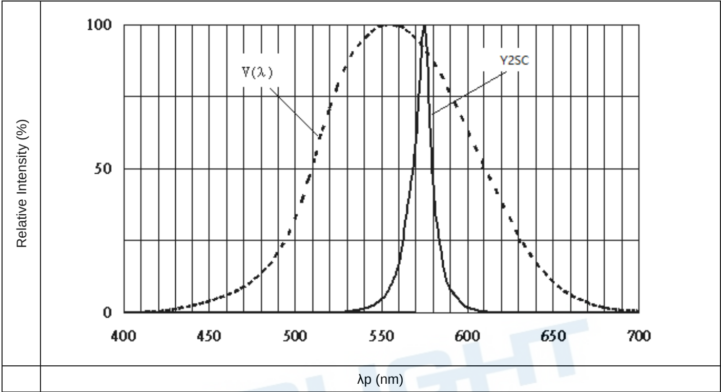
Typical Curve of Spectral Distribution
