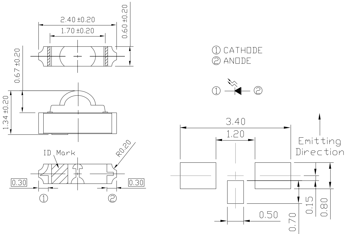
Recommended Soldering Pattern for Side Looker
