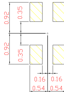
Soldering patterns
