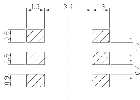
Soldering patterns
