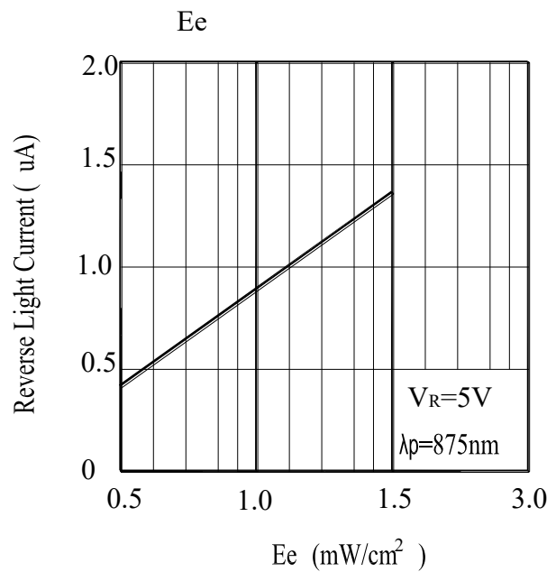
Fig.2 Reverse Light Current vs.
