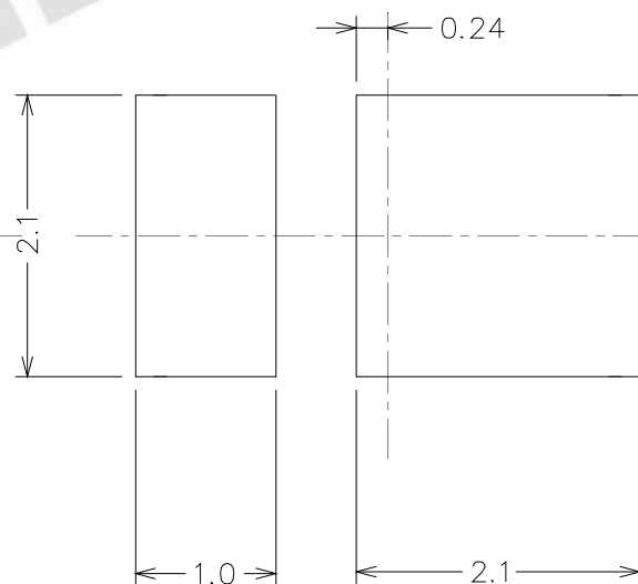
Soldering patterns
