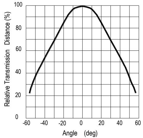
Fig.-5 Relative Transmission Distance vs. Angle
