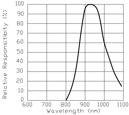
Fig.-4 Relative Spectral Sensitivity vs. Wavelength Direction
