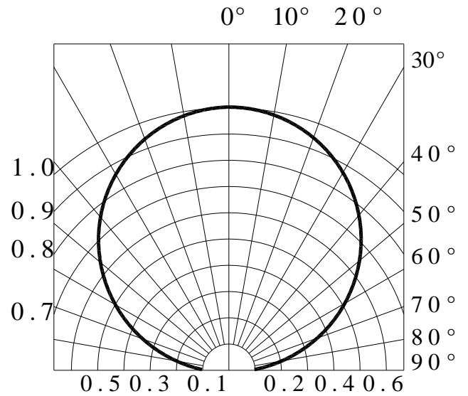
Fig.6 - Radiation Diagram
