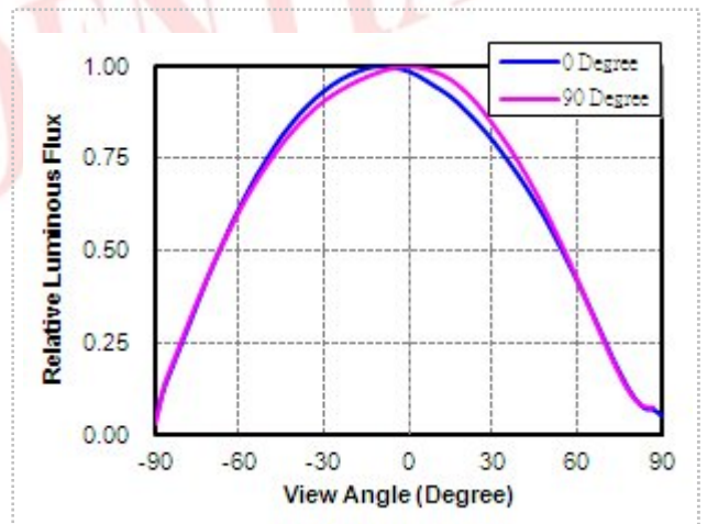
4. Radiation Diagram ( T_s=25^\circ\text{C} , I_f=20\text{mA} )
