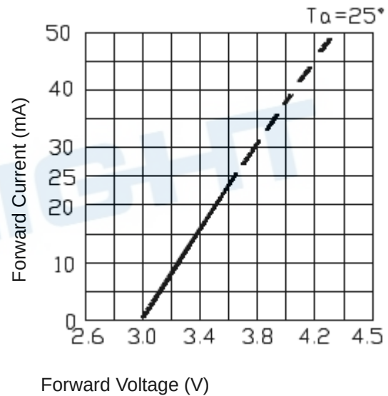
Forward Current vs. Forward Voltage ( T_a = 25^\circ\text{C} )
