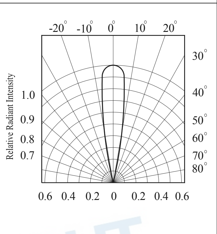
Relative Radiant Intensity vs. Angular Displacement
