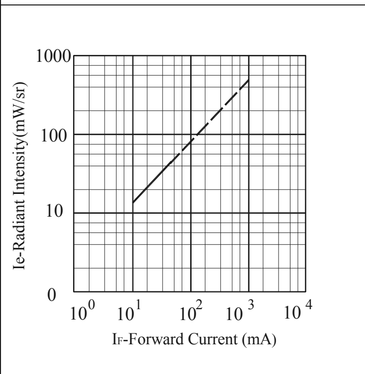
Radiant Intensity vs. Forward Current
