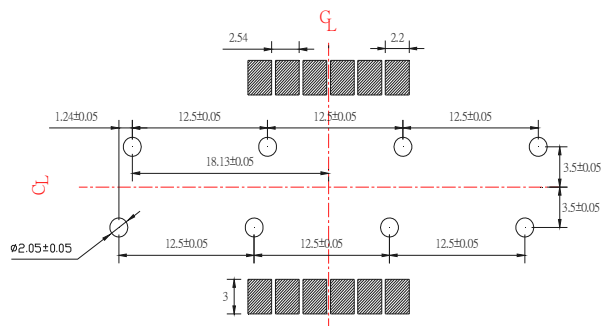
1.2 (B) Recommend soldering pad
