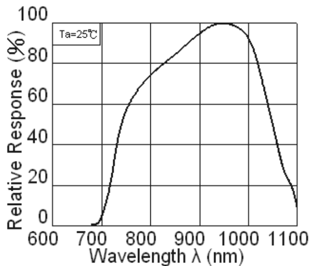
Fig.1 Spectral Sensitivity
