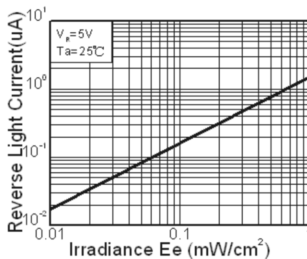
Fig.2 Reverse Light Current vs. E_e
