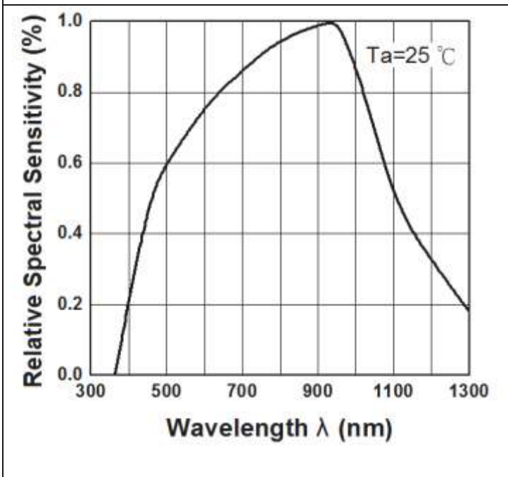
Spectral Sensitivity
