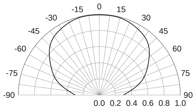
Fig. 11 Horizontal Directivity
