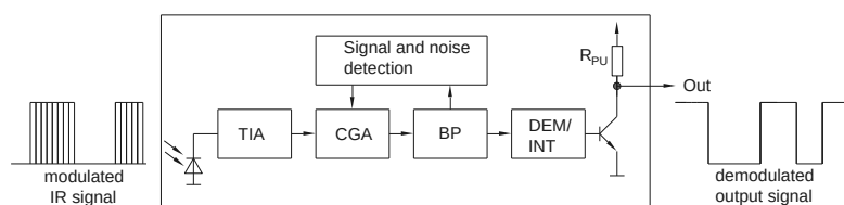
Fig.1 Block Diagram
