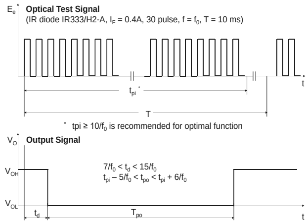
Fig. 5 IR Signal vs. Output Signal
