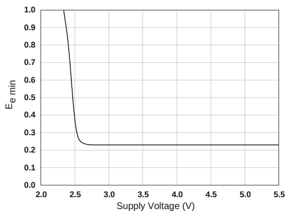
Fig. 8 E_{e\text{ min.}} vs. Supply Voltage
