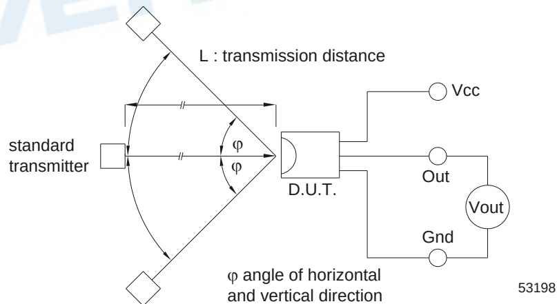
Fig.3 Measuring System
