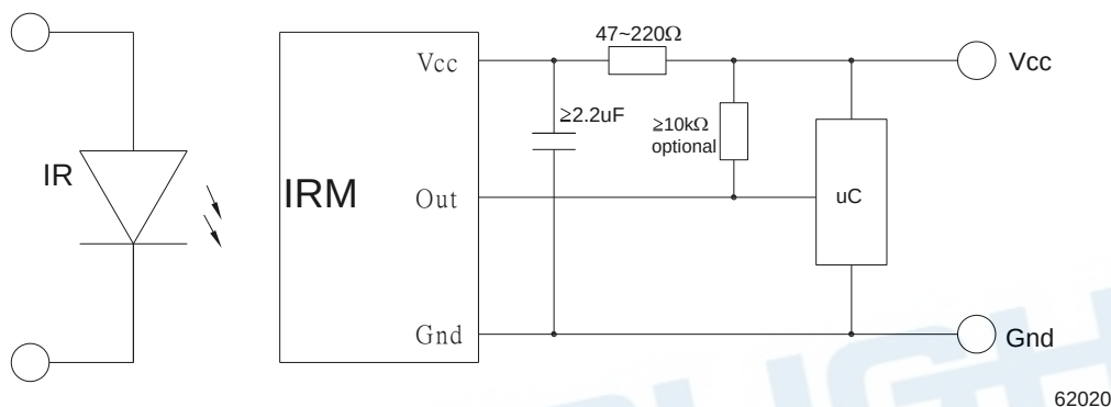
Fig.13: application circuit
