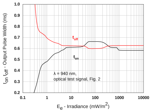
Fig. 10 Output Pulse Diagram
