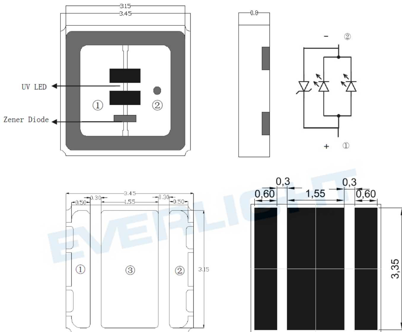
Soldering patterns
