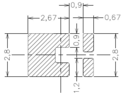
Soldering patterns
