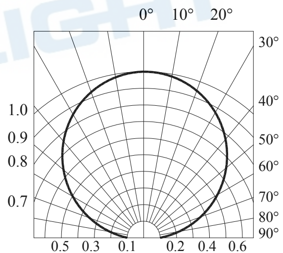
Fig.6 - Radiation Diagram
