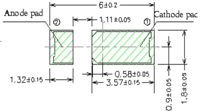
Soldering patterns
