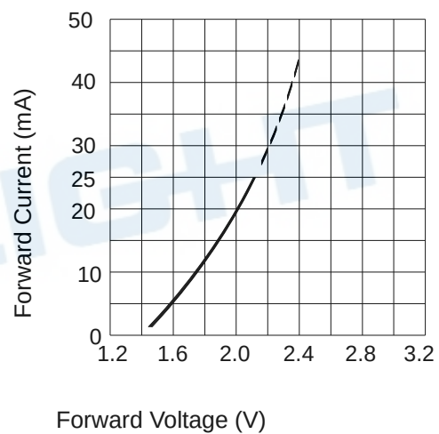
Forward Current vs. Forward Voltage ( T_a = 25^\circ\text{C} )
