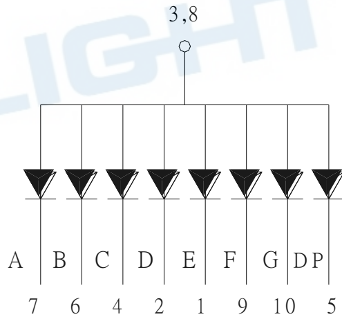
Internal Connection Diagram
