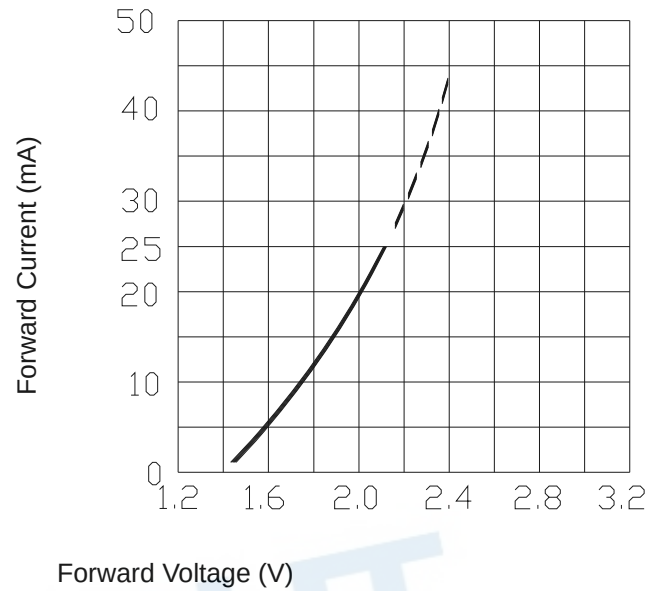
Forward Current vs. Forward Voltage (Ta=25°C) (Per Chip)
