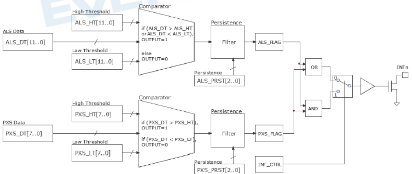
Figure 6. Interrupt operation
