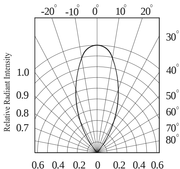
Relative Radiant Intensity vs. Angular Displacement
