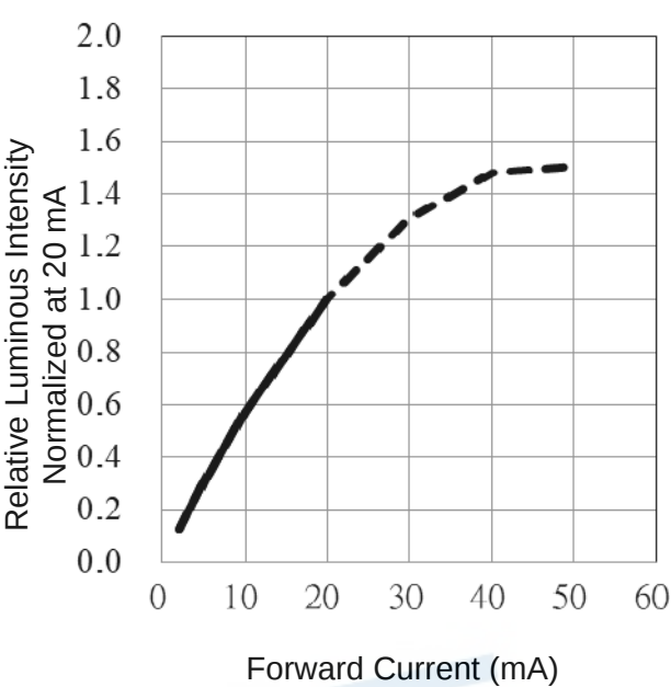
Relative Luminous Intensity vs. Forward Current
