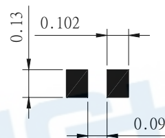
Recommend Soldering Pattern
