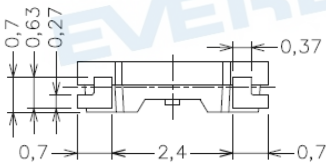
Bot. view
