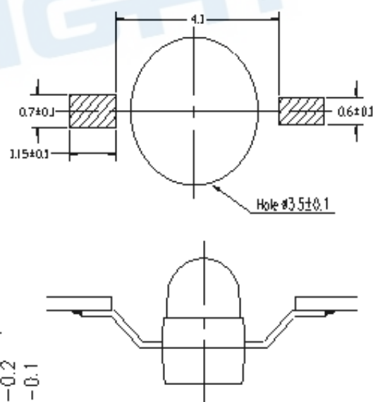
Recommend Soldering Pad
