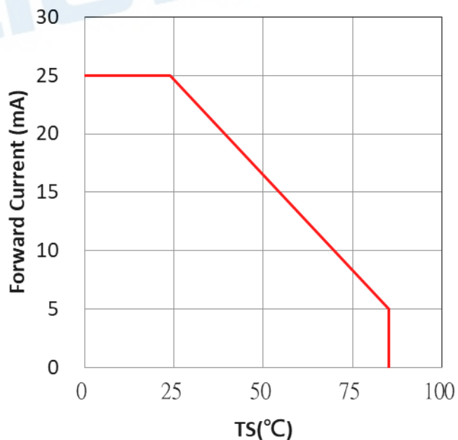
Max. Permissible Forwarded Current (Ta=25°C)
