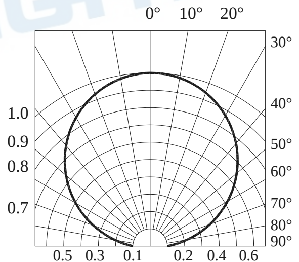
Fig.6 - Radiation Diagram
