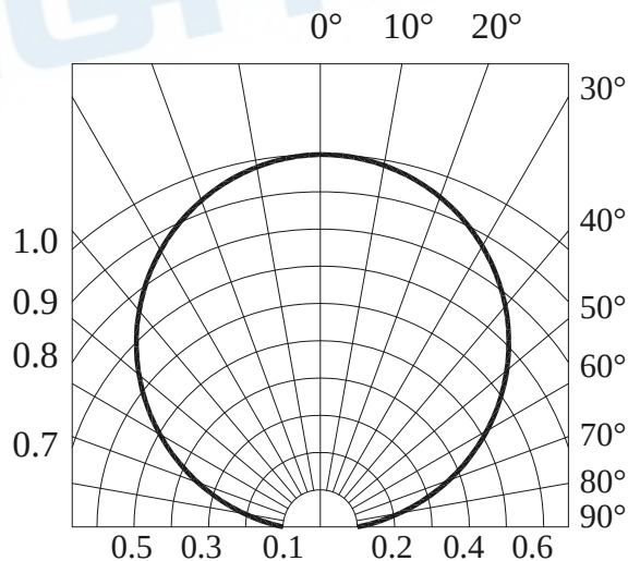
Fig.6 - Radiation Diagram
