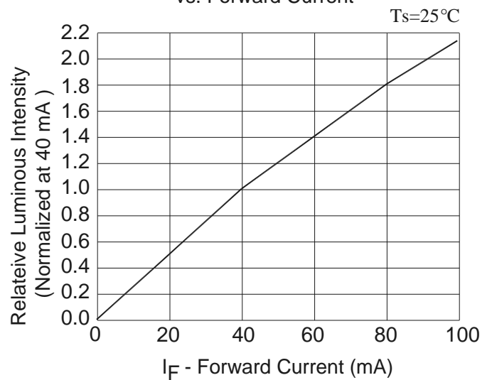
Fig.2 - Relative Luminous Intensity vs. Forward Current
